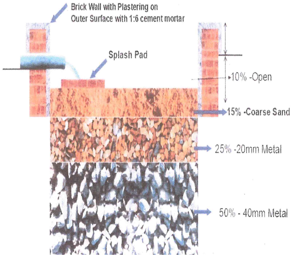
Diagram of Rain Water Harvesting Filter
